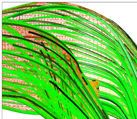
Figure 2: A close-up view of the intake ports in the same CFD simulation grid as shown in figure 1. We can see multiple, adaptive resolution levels of unstructured grid cells.
