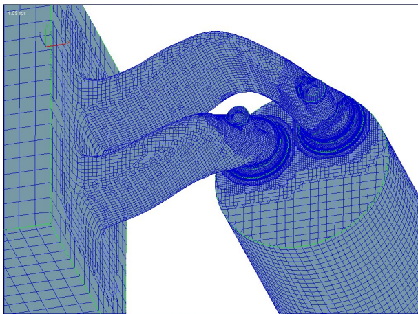
Figure 1: The CFD simulation grid of an intake port. This image illustrates the versatility of a typical, unstructured, CFD simulation grid containing a flow source from the left, two connecting pipes in the middle, two intake ports at the ends of the pipes, and a combustion chamber cylinder on the right ( intake port data courtesy of AVL ).
