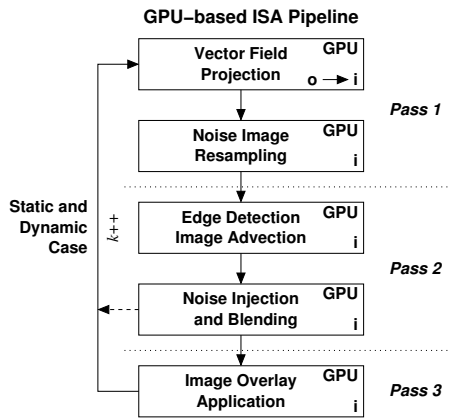
Figure 2: The major components of the GPU-based ISA implementation. While all stages are performed at each frame, the output of the final stage is only displayed to the user. The data feedback loop is closed at the noise injection and blending stage, which is indicated by the dashed arrow (see Section 3.5).
